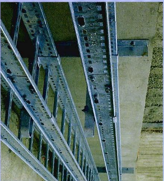
M12 Screwbolts fixing cable tray brackets throughout tunnel
